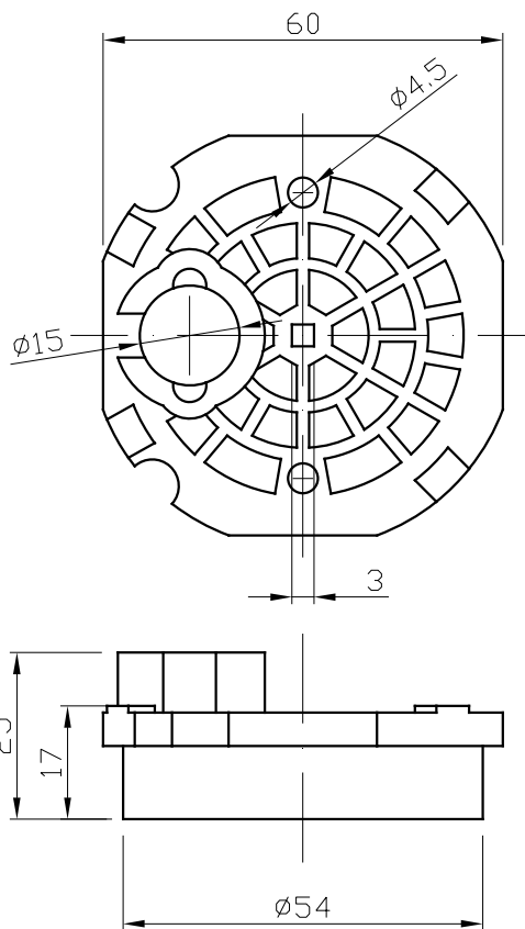
2-HEAD BLOWER SUPPORT D54x25 MATERIAL: CERAMIC
