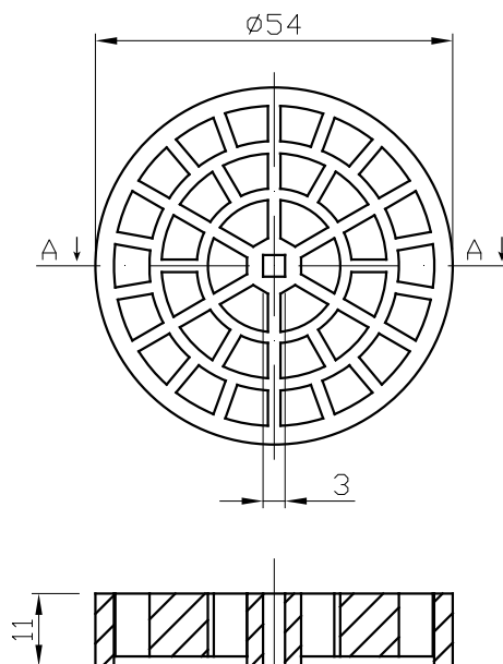
3-BOTTOM BLOWER SUPPORT D54x11 MATERIAL: CORDIERITE
